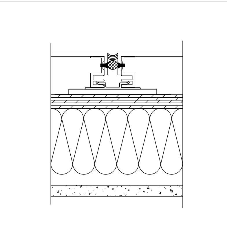
3 310 COPING PANEL JOINT SCALE: NTS
