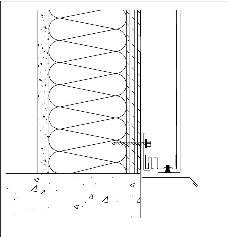
1 310 FOUNDATION SCALE: NTS
